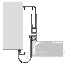
EUROFI-E Eckzarge
